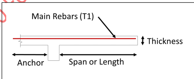
Figure 13 – Cantilever slab.
