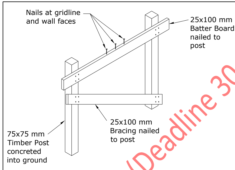
Figure 4 – Batter boards.
