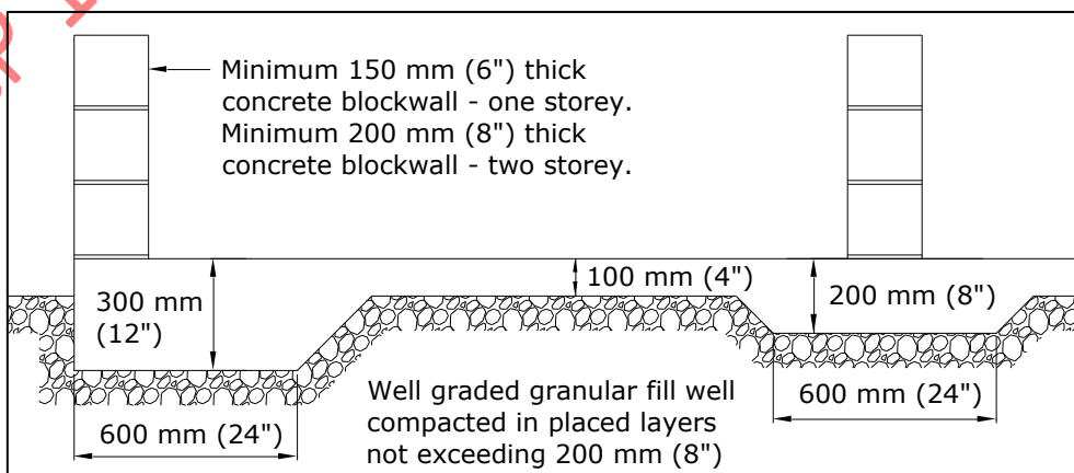
Figure 7 – Layout of slab-on-ground footing.
